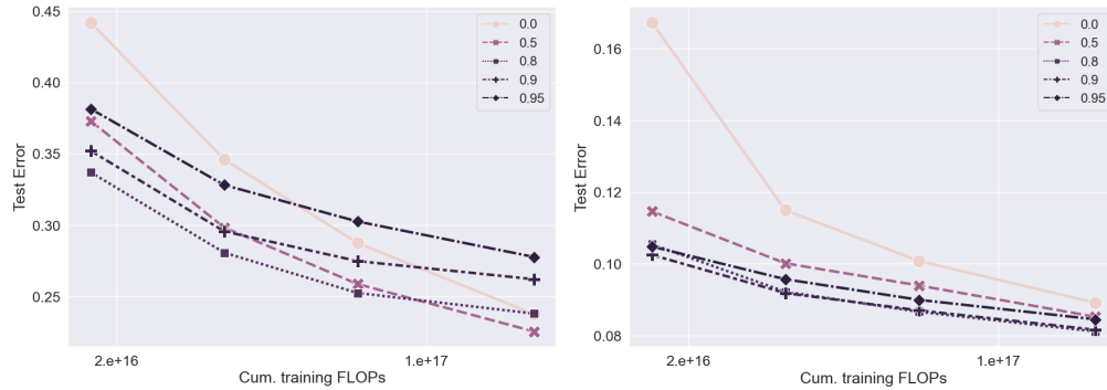
(a) Transfer Learning - Object
